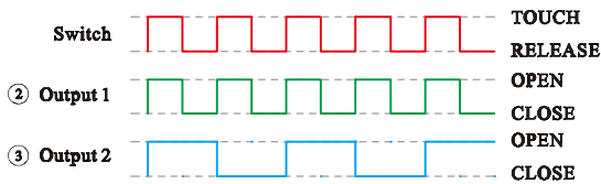
Function Type A LED external control
