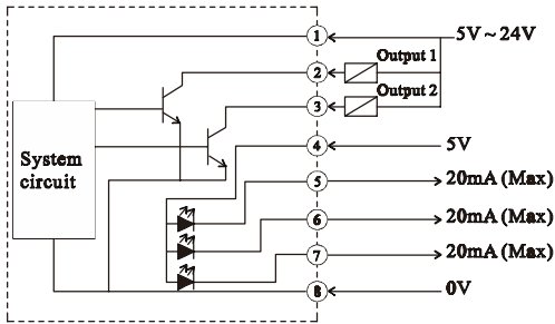
Function Type A LED external control
