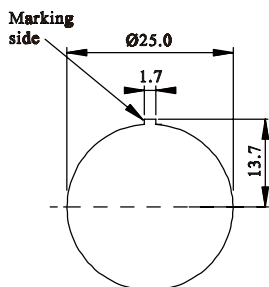
Panel cutting Panel thickness 1.5~4mm
