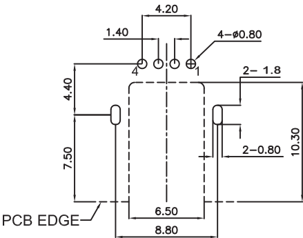
RECOMMENDED PCB LAYOUT TOP VIEW TOLERANCE:±0.05mm PCB THICKNESS: 1.00±0.05mm
