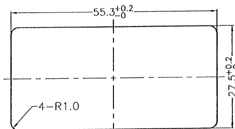
PANEL CUT-OUT
