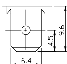
TERMINAL TYPE
