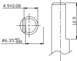
SHAFT TYPE
