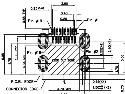
RECOMMENDED PCB LAYOUT TOP VIEW TOLERANCE:±0.05mm PCB THICKNESS: 0.80±0.05mm
