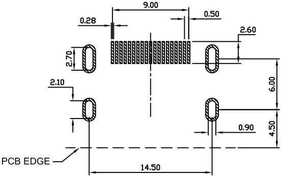
SUGGESTED PCB LAYOUT TOP VIEW
