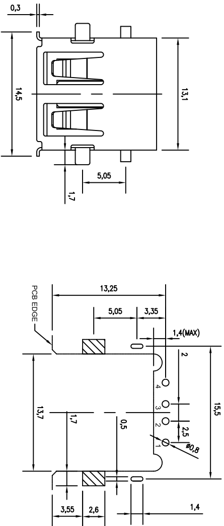
RECOMMEND PCB LAYOUT TOP VIEW
