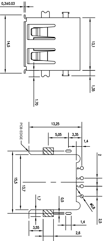
RECOMMENDED PCB LAYOUT TOP VIEW
